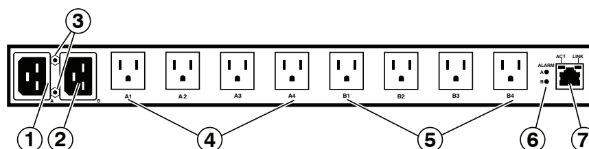
Figure 2.6: NPS-8HD Series - Back Panel
